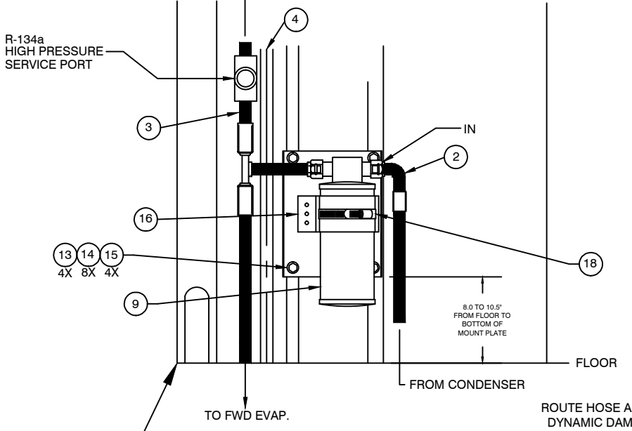
VIEW B-B
