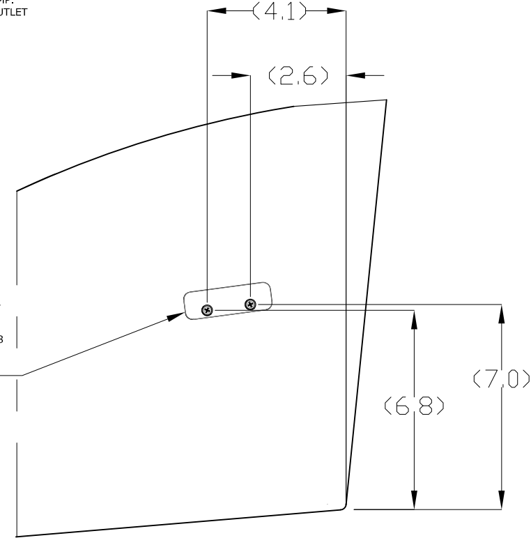
SECTION B-B GLARE SHIELD REFERENCE AIR VENT REMOVED FOR CLARITY (VENT LOCATION SHOWN AS APPROXIMATE)
