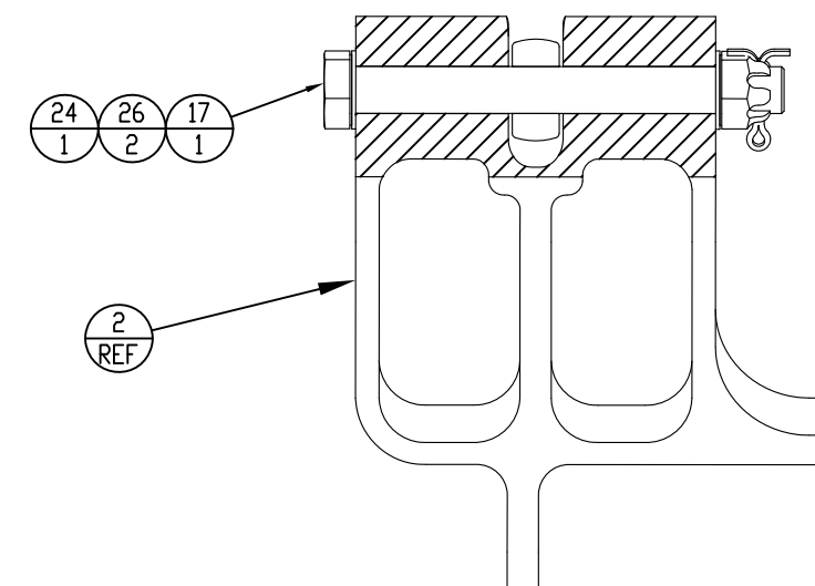
SECTION H-H \triangle 6 (SHOWN WITH COTTER PIN TYPE HARDWARE)
