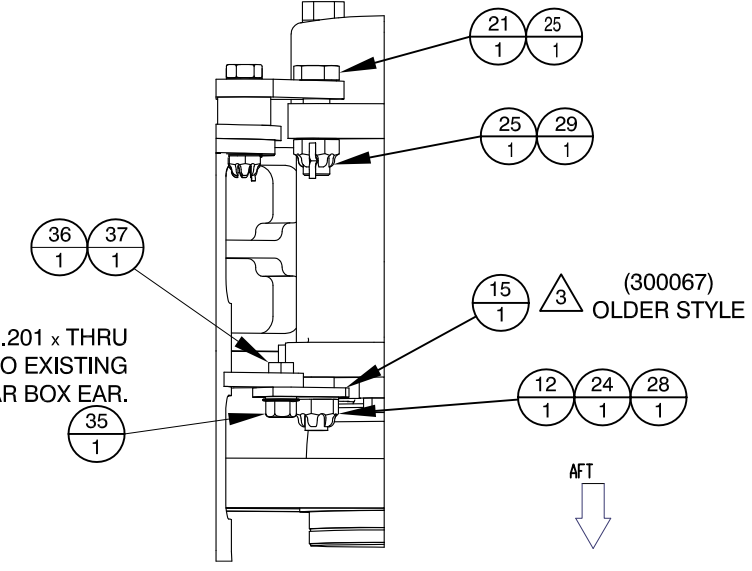
SECTION F-F (VIEW LOOKING UP.) (SHOWN WITH COTTER PIN TYPE HARDWARE)
