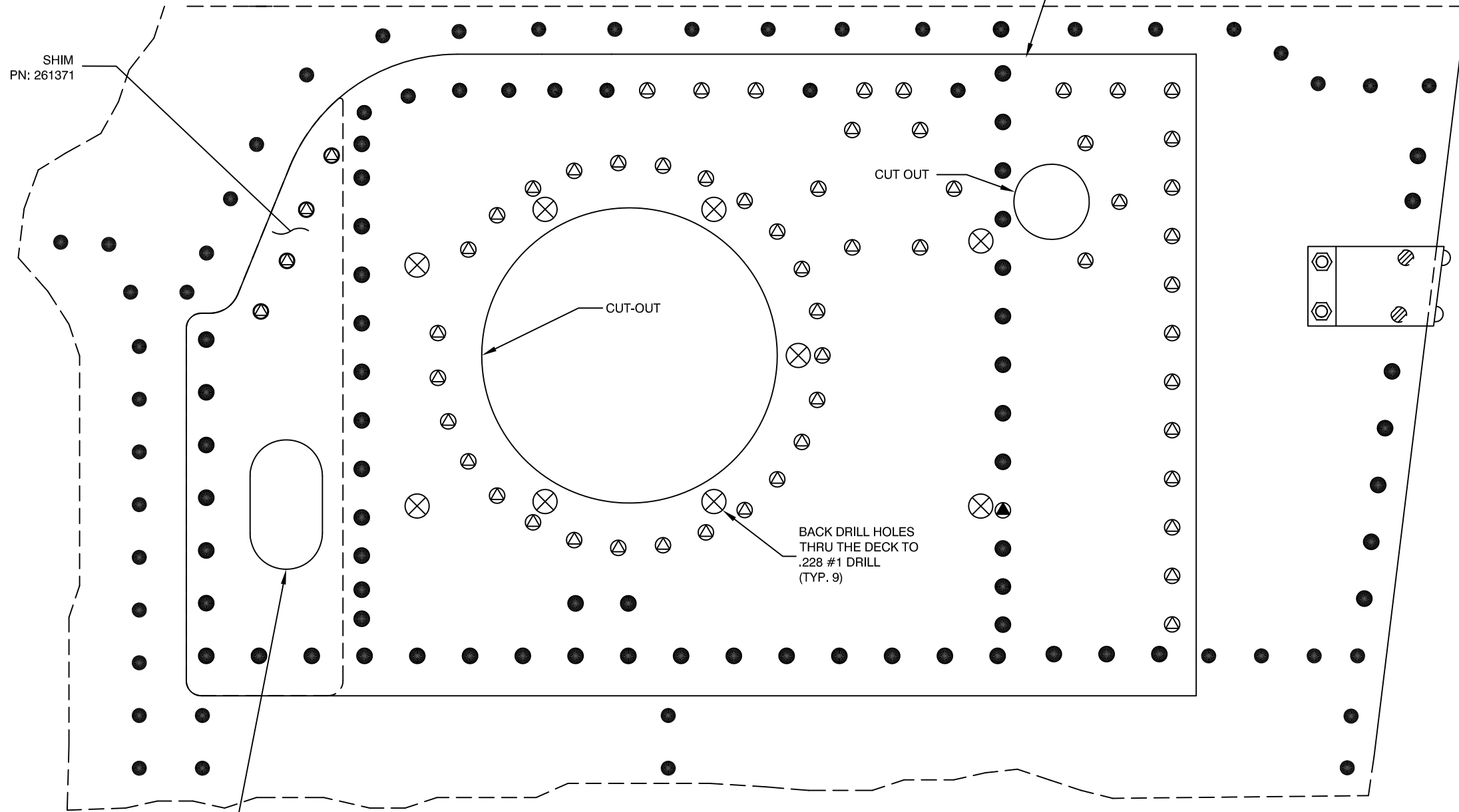
VIEW LOOKING DOWN AT TRANSMISSION DECK
