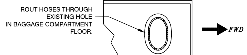
VIEW D-D VIEW LOOKING DOWN
